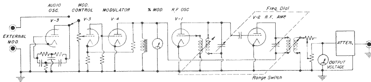
Figure 1. Elementary Schematic Diagram.
