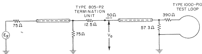
Figure 2. Diagram of Type 1000-P10 Test Loop.
