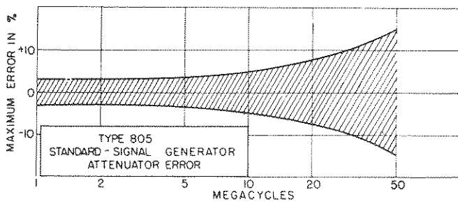
Figure 7. Maximum attenuator error as a function of frequency.
