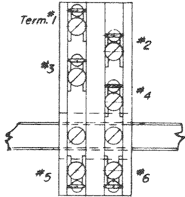
Figure 4. Identification of terminals on terminal blocks of r-f inductors.
