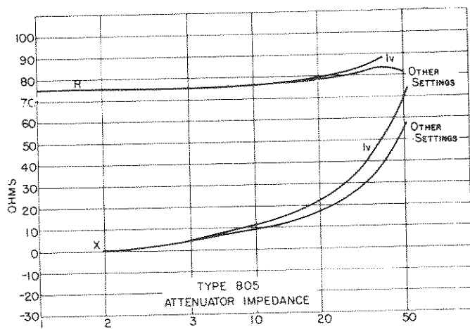
Figure 11. Attenuator impedance as a function of frequency.
