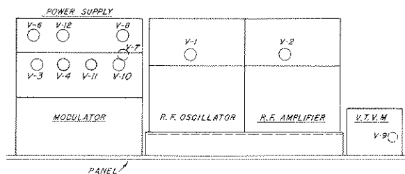
TOP VIEW OF INSTRUMENT TUBE LAYOUT
