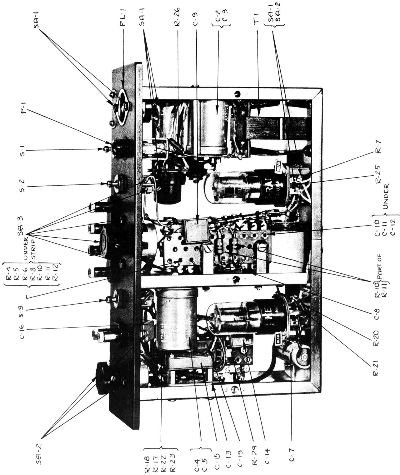
Figure 4. View of Type 650-P1 with Covers Removed.
