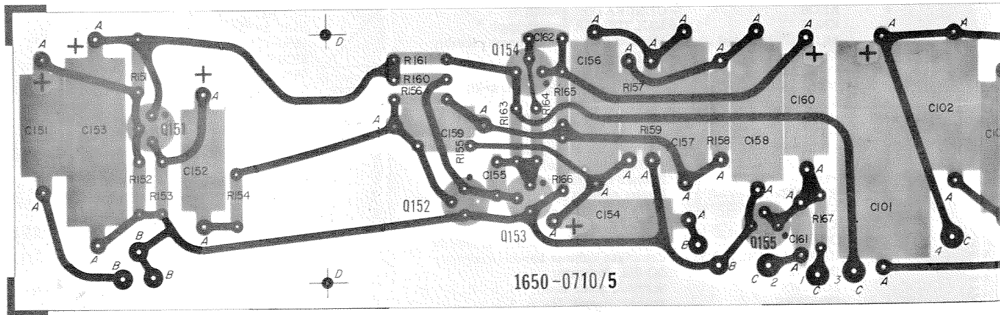
Figure 6 - 4. Etched circuit assembly (P/N 1650-2710).
