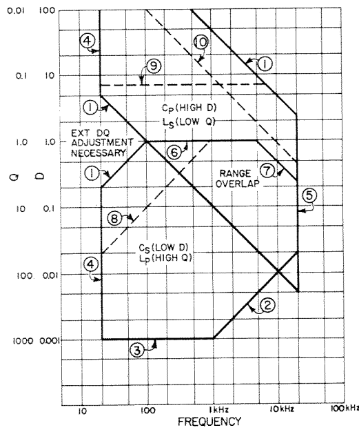
Figure 4-5. DQ ranges vs frequency.
