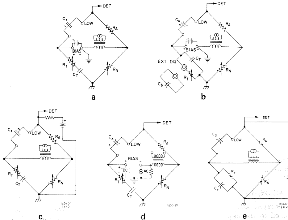
Figure 3-1. Methods of applying dc voltages to capacitance.
