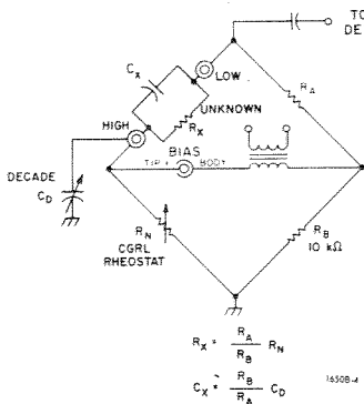
Figure 3-6. Circuit for measuring capacitive resistors.
