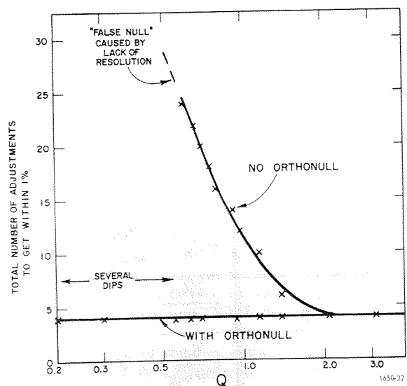
Figure 4-3. Number of balances vs Q.
