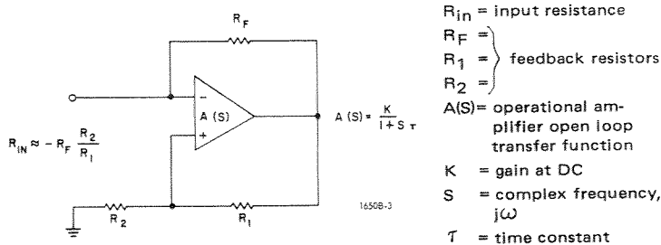
Figure 3-5. Operational amplifier.
