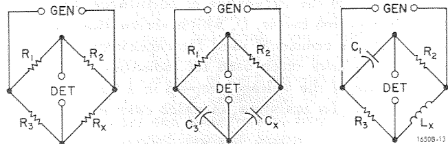
Figure 5-1. The general Wheatstone bridge circuit. Figures 5-2 and 5-3. Circuits for capacitance bridges in which like reactances (left) or unlike reactances (right) are compared.
