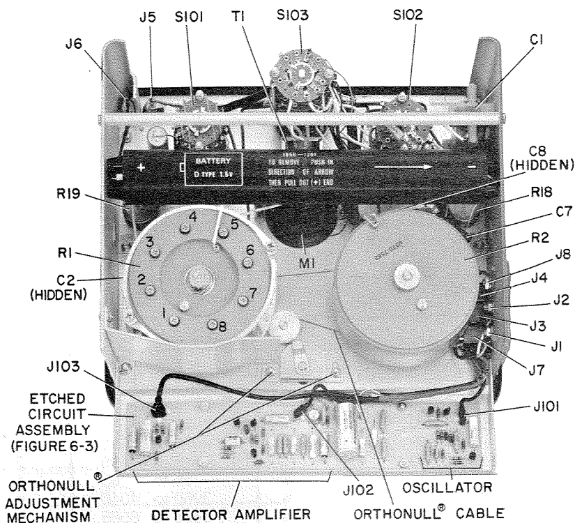
Figure 6 - 2. Interior view of 1650-B Bridge.
