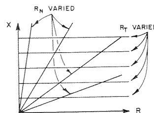
Figure 5-7. Loci of R_N and R_T adjustments on Z plane.
