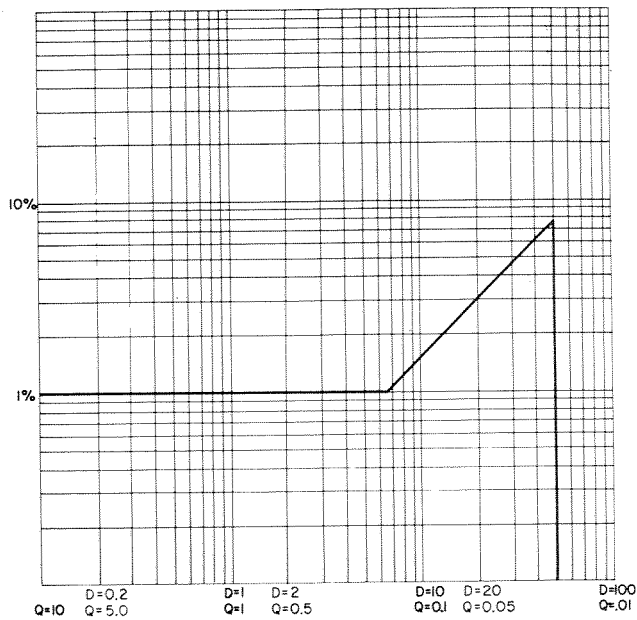
Figure 4-4. Accuracy vs D or Q.
