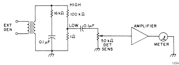
Figure 6 - 3. Schematic for checking the detector circuit.
