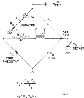
Figure 3-7. Circuit for measuring inductive resistors.
