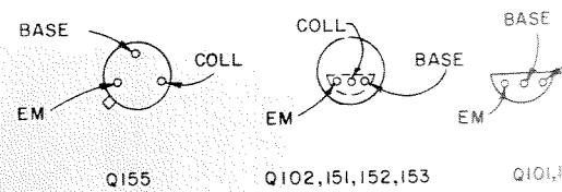
BOTTOM VIEW OF TRANSISTORS
