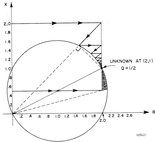
IDEALIZED BALANCING LOCI Q = 1/2 Figure 5 - 8. Loci of "sliding null" balance.
