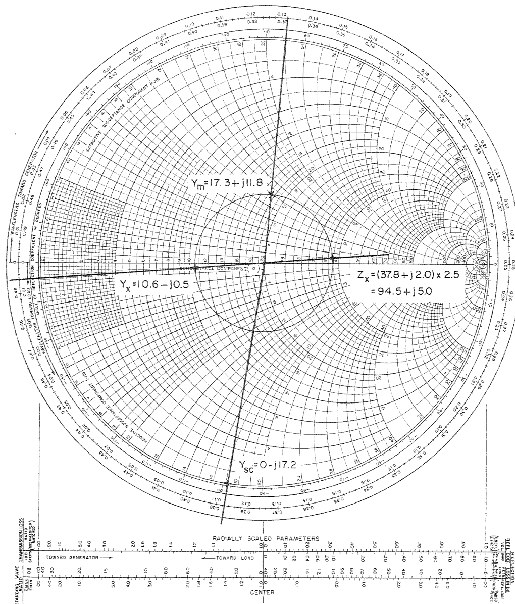
Figure 14. The use of the Smith Chart to calculate the admittance and impedance of a resistor from values measured on the Admittance Meter.
