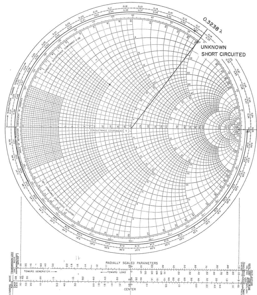
ADMITTANCE COORDINATES—20-MILLIMHO CHARACTERISTIC ADMITTANCE
