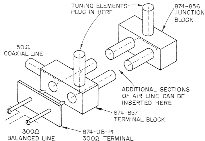
Figure 10. Schematic showing function arrangement of balun.
