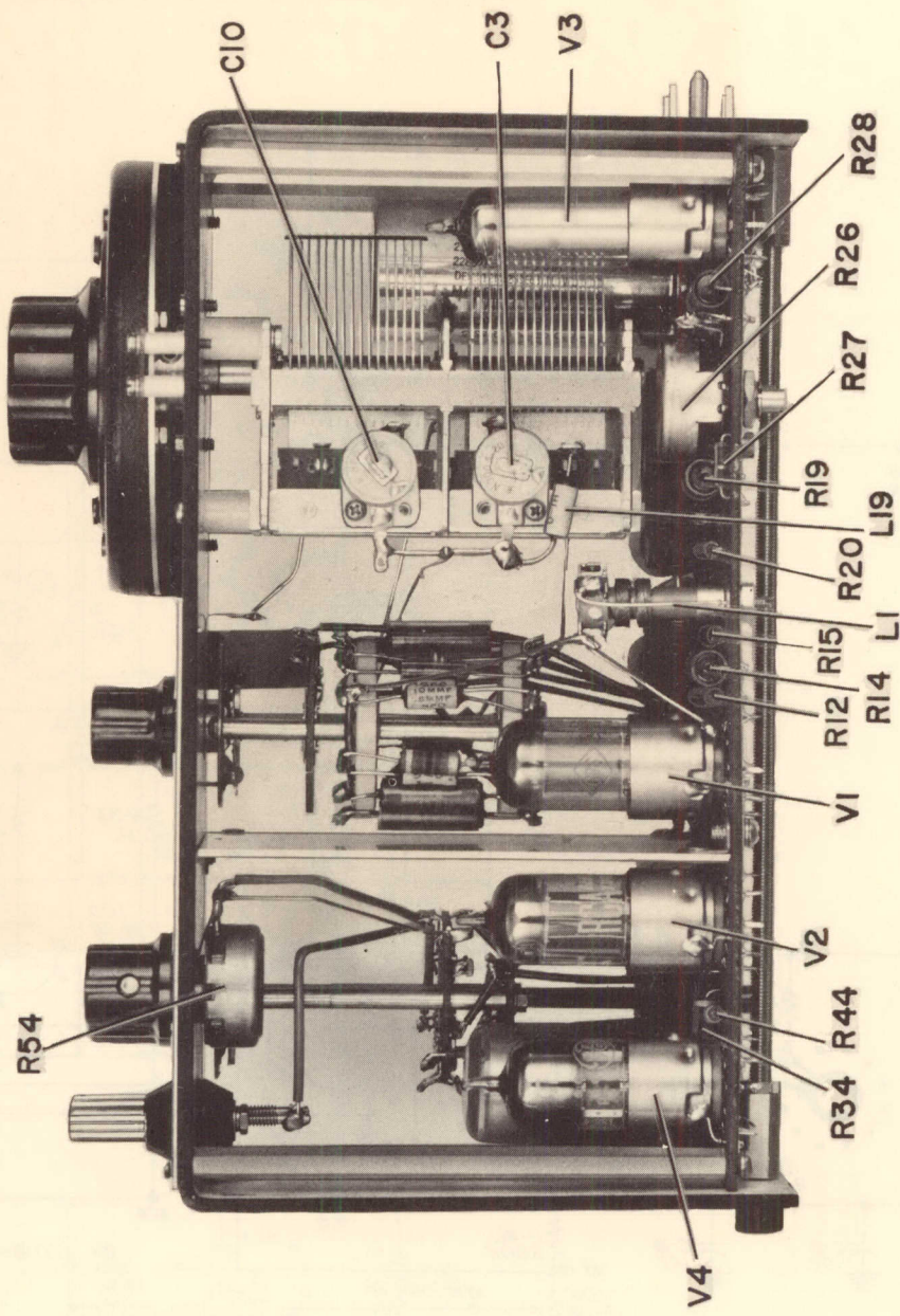
Figure 5. Top Interior View of Type 1210-C Unit R-C Oscillator.
