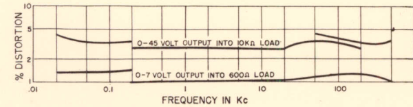
Typical output and harmonic distortion characteristics of the Type 1210-C Unit RC Oscillator as functions of frequency and load.
