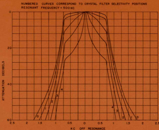
1.4 kc Mechanical Filter Selectivity Curves
