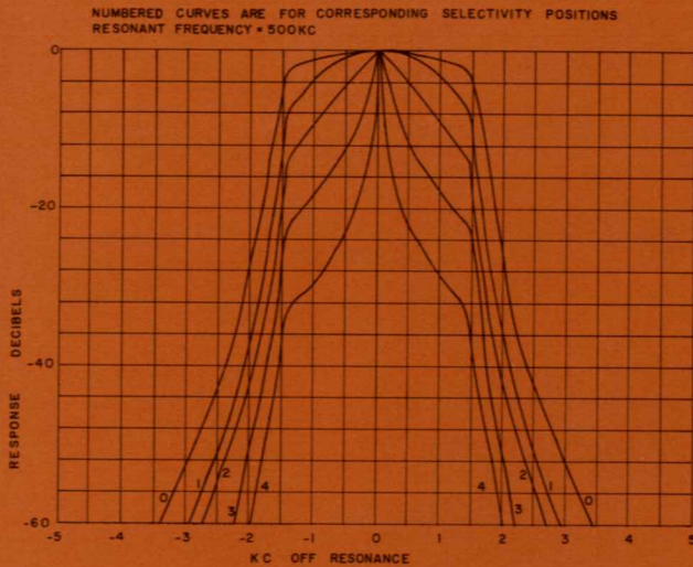
3 kc Mechanical Filter Selectivity Curves
