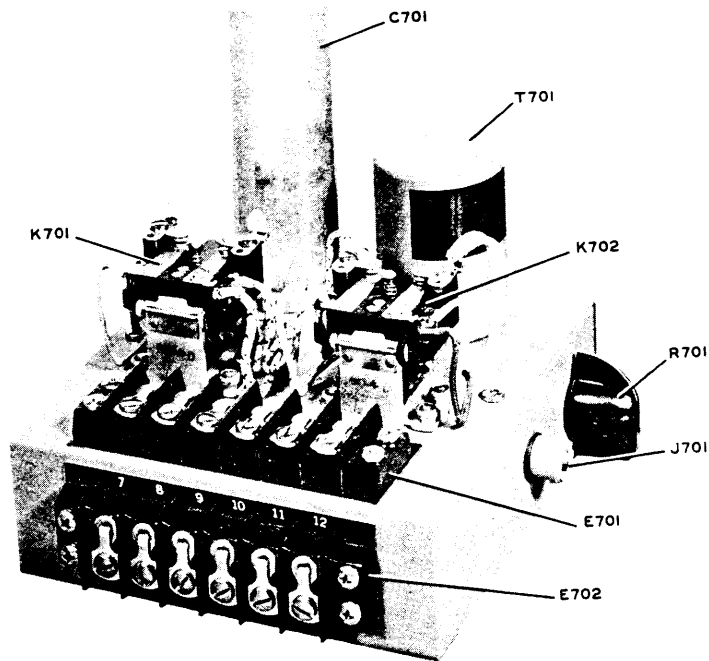
Figure 5-11. Type 175V-2 Relay Unit, Parts Arrangement - Top
