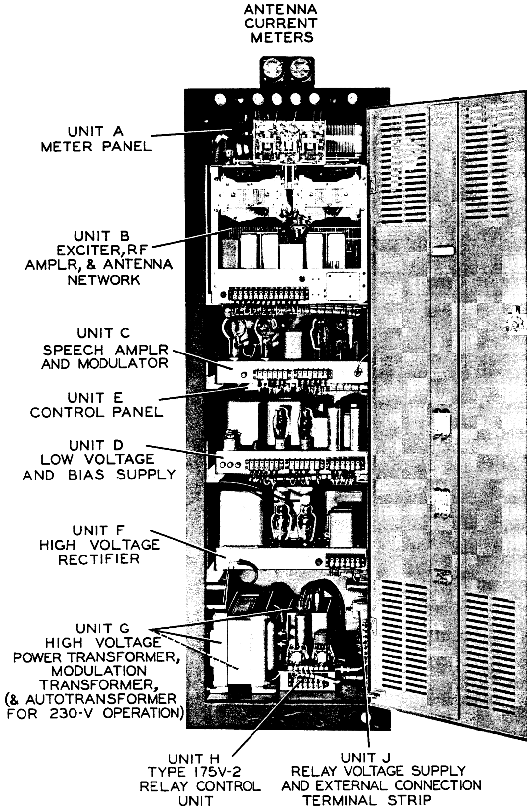
Figure 2-3. Unit Placement Photograph
