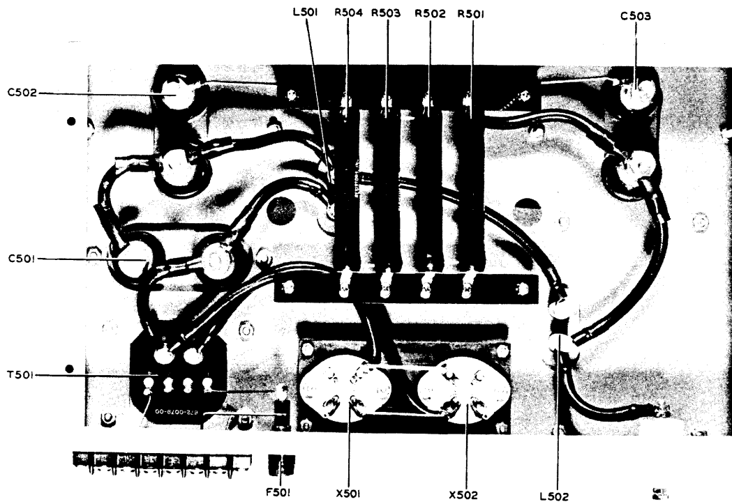
Figure 5-10. High Voltage Rectifier and Filter, Parts Arrangement - Bottom
