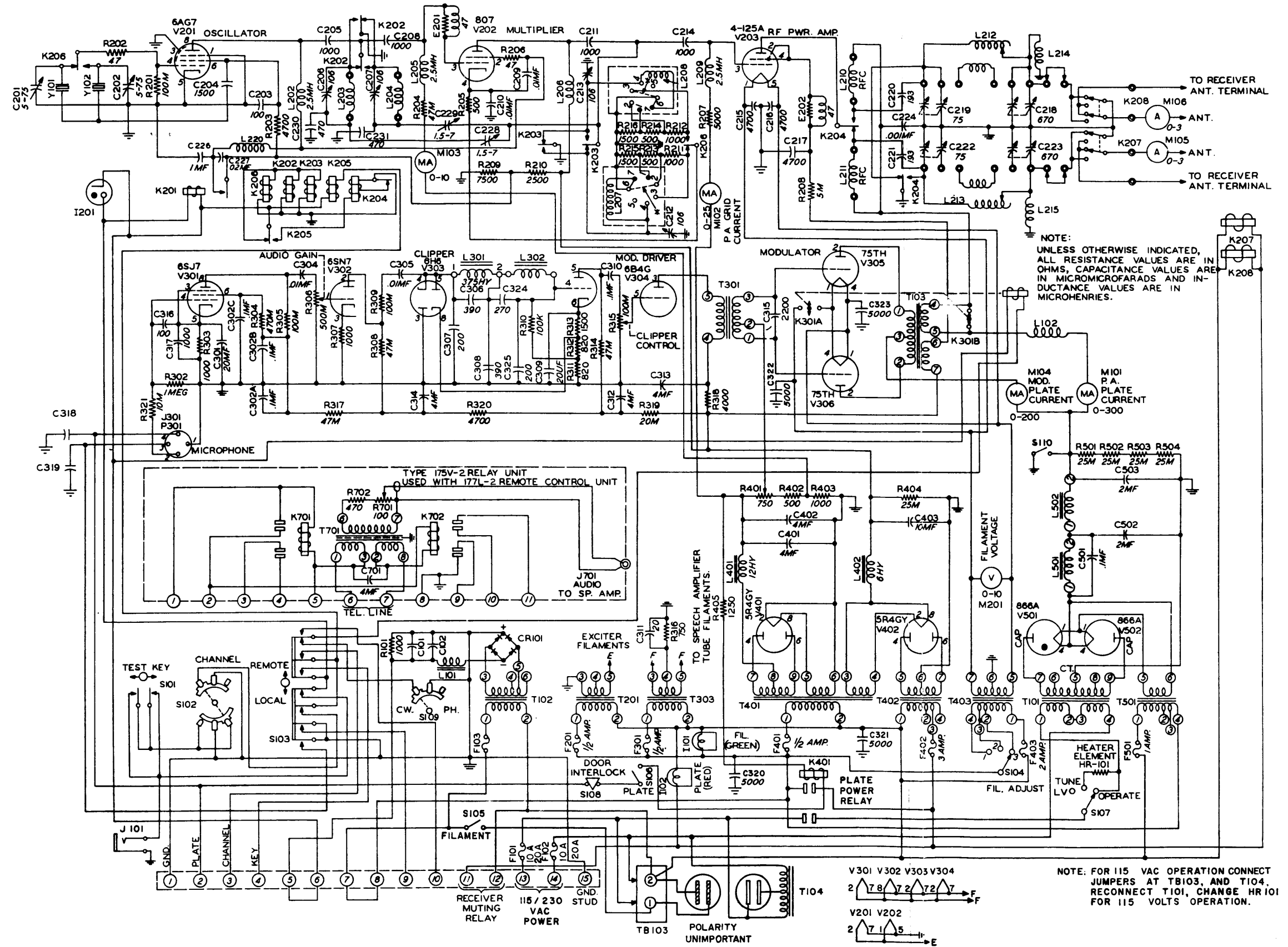
Figure 5-15. Type 30K-5 Transmitter, Complete Schematic (Shown Wired for 230-V Operation)
