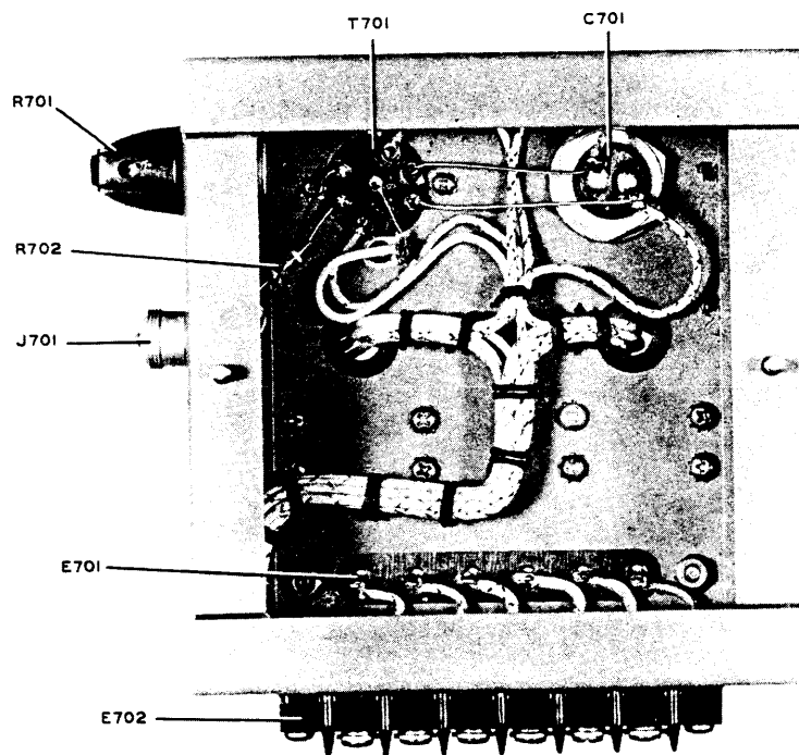
Figure 5-12. Type 175V-2 Relay Unit Parts Arrangement - Bottom
