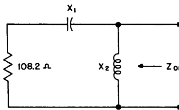
Figure 7-2. Equivalent Circuit, 108.2 ohms to Z_{01}
