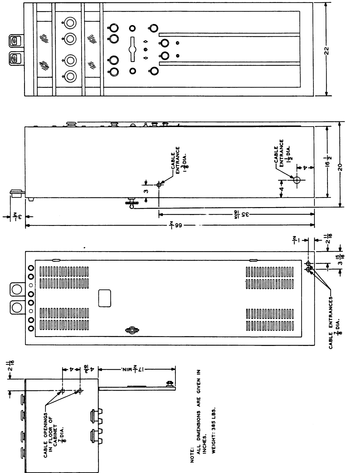
Figure 2-1. Type 30K-5 Transmitter Outline and Mounting Dimensions
