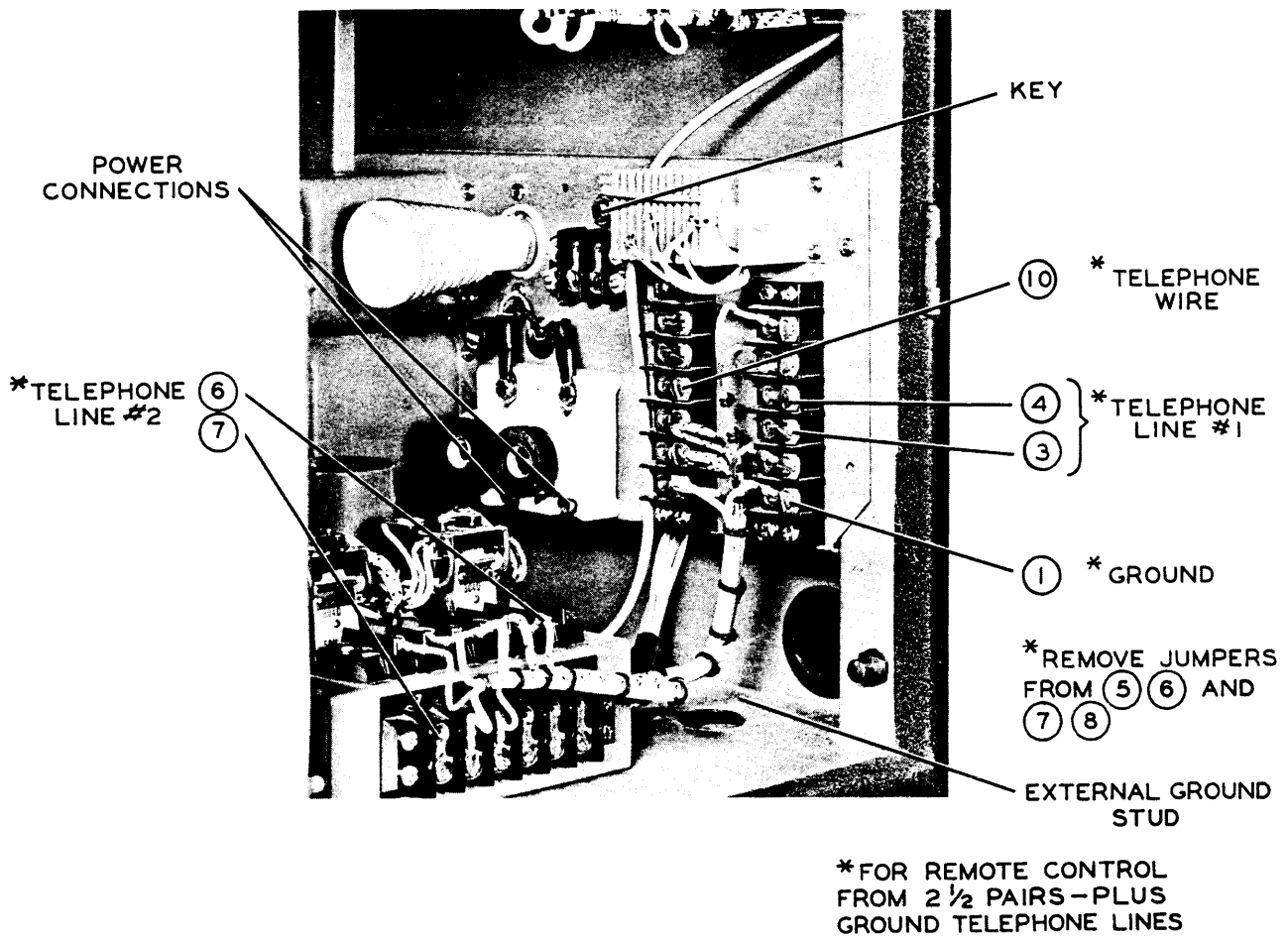
Figure 2-4. External Connections
