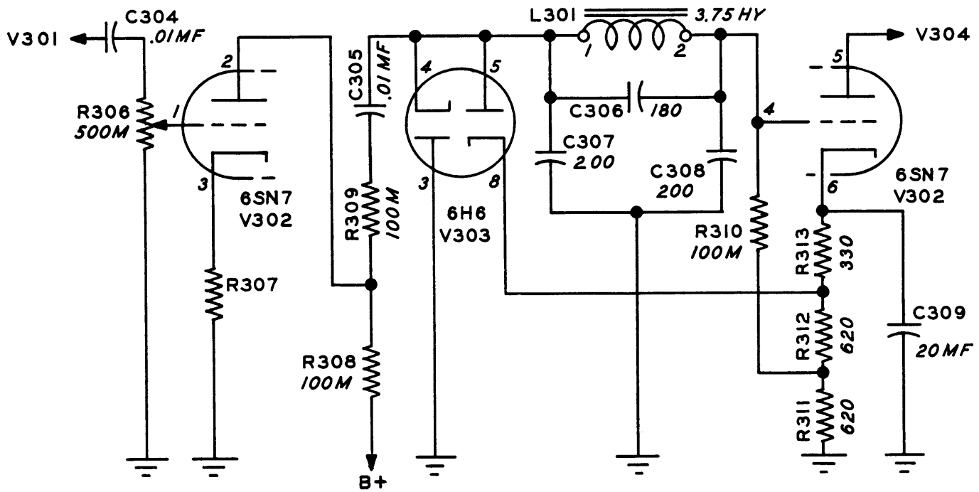
Figure 4-3. Audio Peak Clipper Circuit
