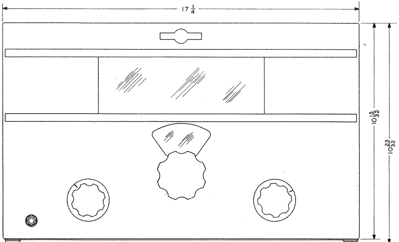
Figure 3-2 Exciter Outline Dimensions
